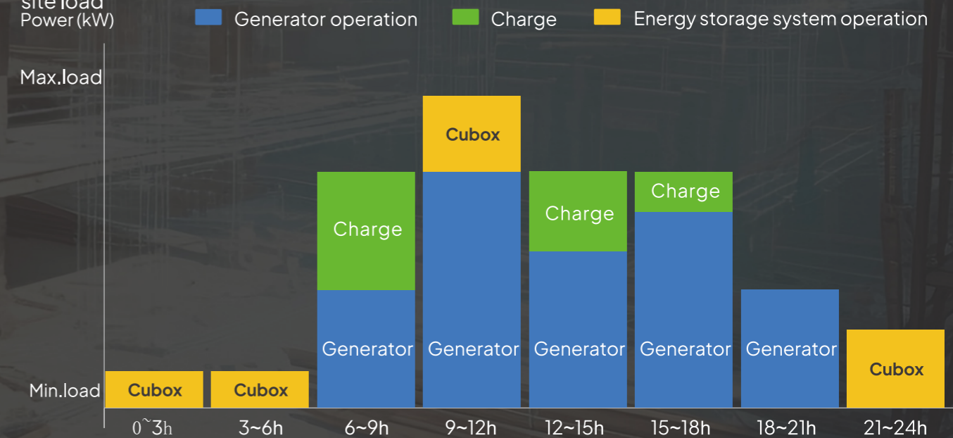
Typical application models at construction sites
